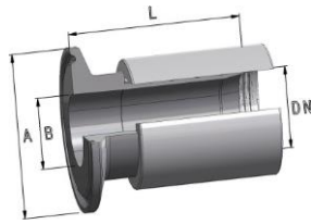
Clamp
